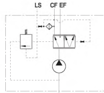
Hidrolik Devre Hydraulic Circle
